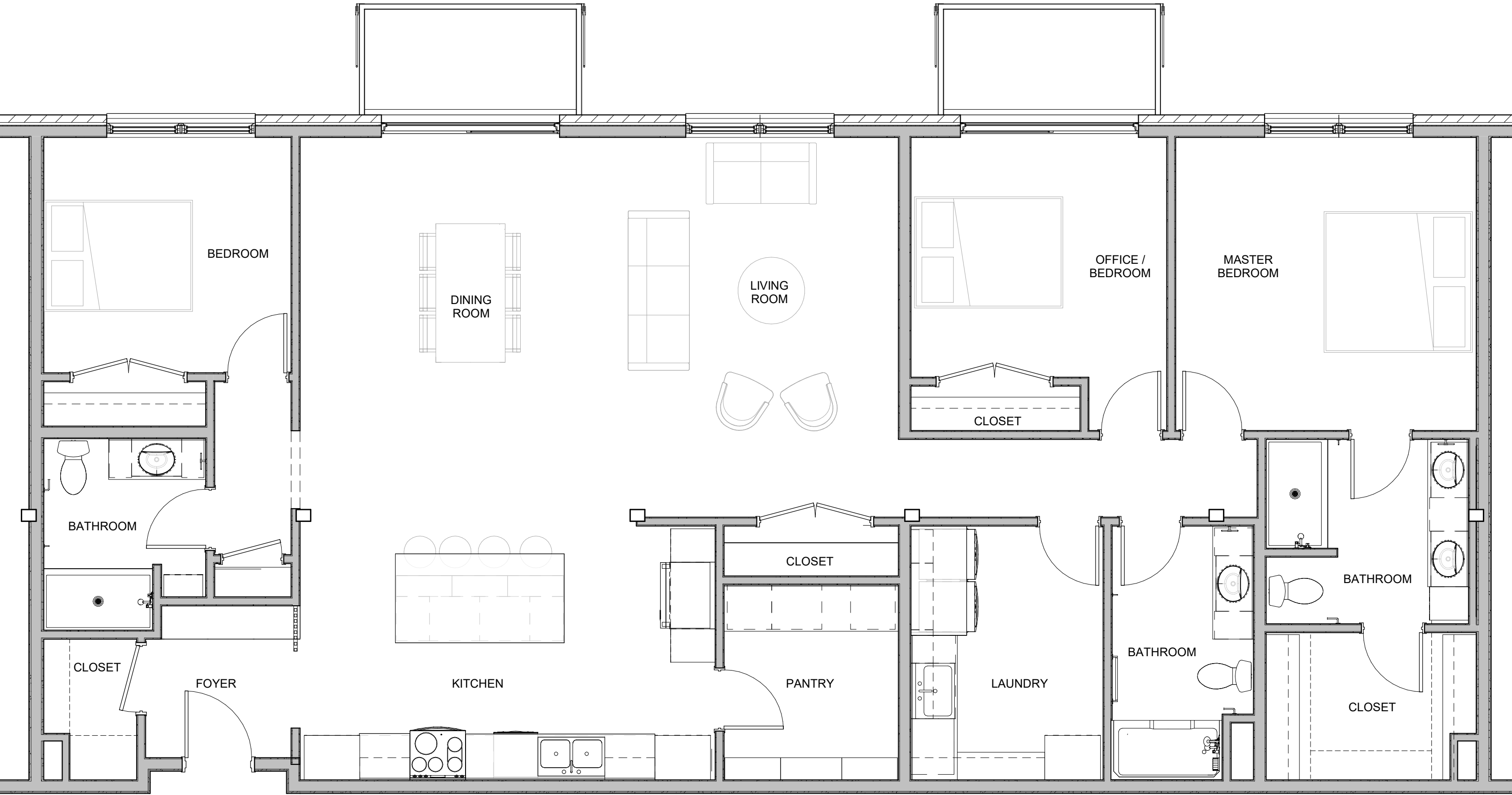
3 BEDROOM UNIT
