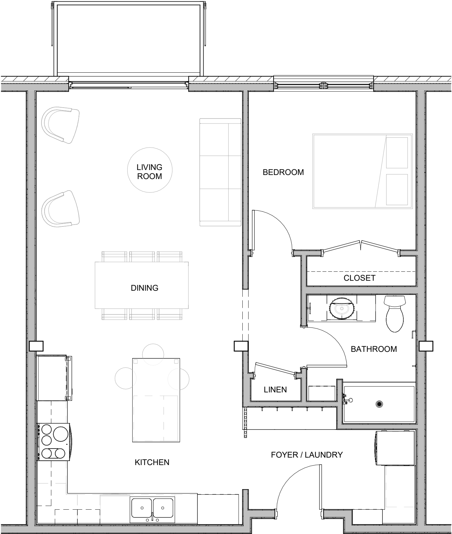
1 BEDROOM UNIT
